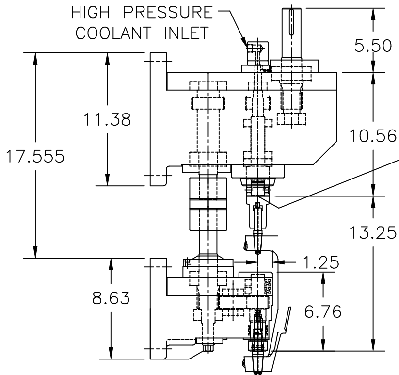
LOWER SPINDLE ASSEMBLY
