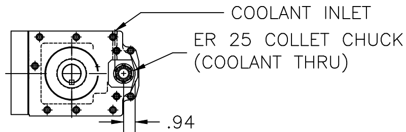
LOWER SPINDLE ASSEMBLY
